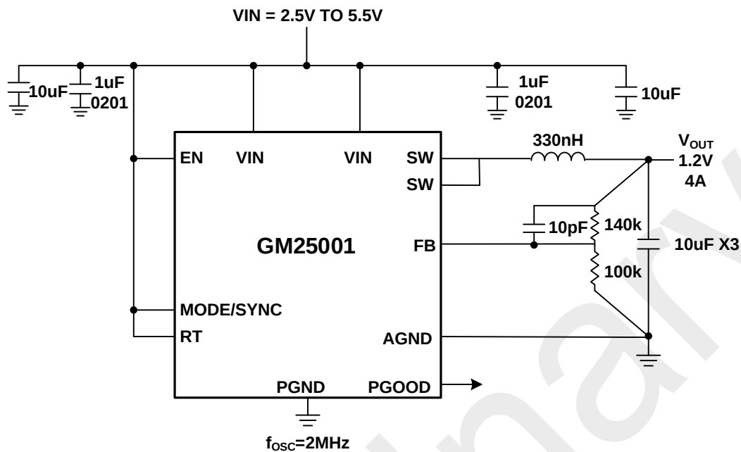
图 27. 2MHz, V IN =3.3V, V OUT =1.2V, I LOAD =4A
