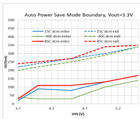
图20. PFM/PWM Boundaries, Mode=Low, V_{OUT} = 3.3V
