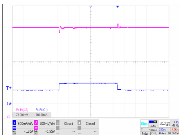
图32. 负载瞬变, V_{OUT} = 1.8V , Mode=High, I_{LOAD}= 500mA to 750mA
