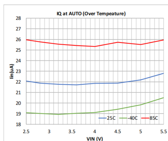
图17. I_Q vs V_{IN} 过热, Mode=Low, V_{OUT} = 1.8V
