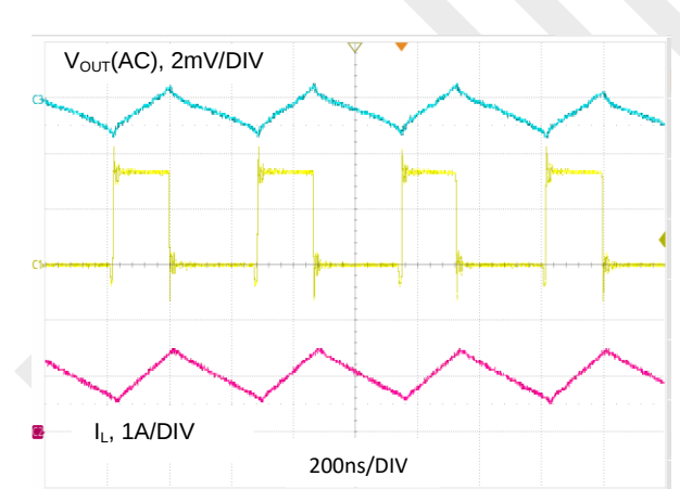
图 14. V_{OUT} = 1.2\text{V} , I_o = 1\text{A} , FPWM
